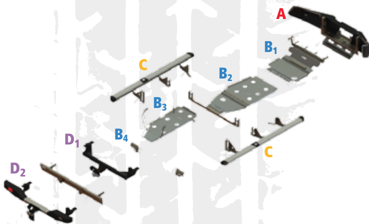
Permanent rear tow bar
